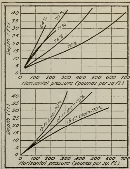
Grass silage pressures at silo wall: (Top) With different moisture contents in 12-foot diameter silos, and (lower) with a 70-percent moisture content in different sized silos.
